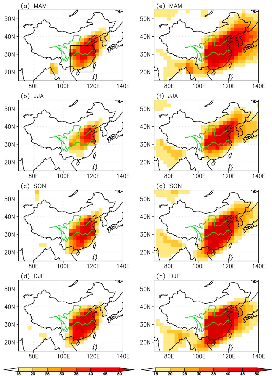
Figure 2. The spatial distribution of the simulated (a–d) surface layer \text{PM}_{2.5} concentrations ( \mu\text{g m}^{-3} ) and (e–h) column burdens of \text{PM}_{2.5} ( \text{mg m}^{-2} ) during the seasonal cycle averaged from 1986 to 2006.
