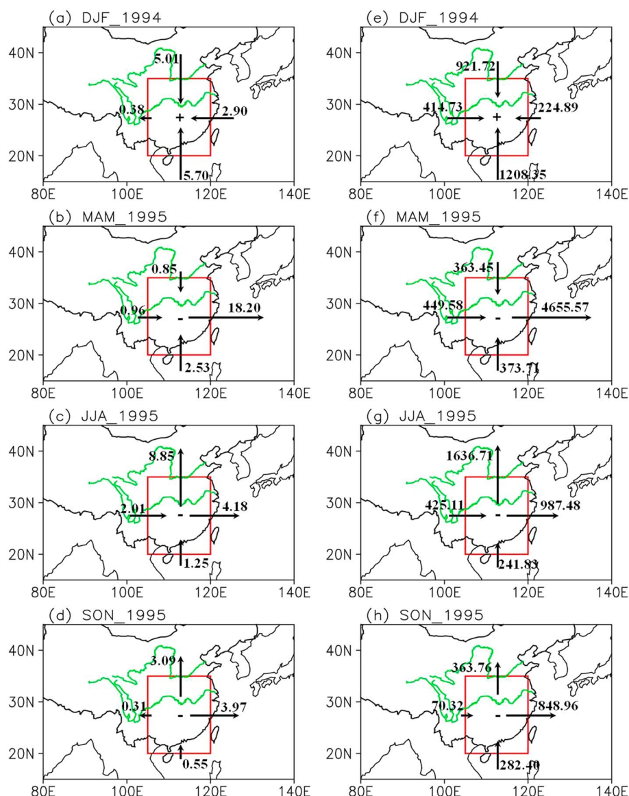
Figure 7. The simulated horizontal budget anomalies of \text{PM}_{2.5} concentration mass fluxes (a–d) at 700 hPa and (e–h) integration within the lower troposphere from 1000 to 700 hPa during El Niño Modoki event 1994/1995 ( \mu\text{g m}^{-3} ).
