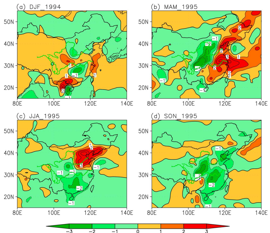
Figure 9. The simulated vertical integral wet deposit flux anomalies during El Niño Modoki event 1994/1995 for (a) mature winter and decaying (b) spring, (c) summer, and (d) autumn ( \text{kg s}^{-1} ).
