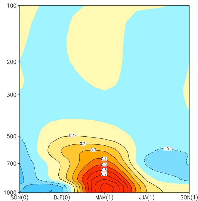
Figure 8. As in Figure 5 but for the pressure-time distribution of simulated \text{PM}_{2.5} concentration upward mass flux anomalies averaged over southern China within 105^{\circ} – 120^{\circ}\text{E} , 20^{\circ} – 35^{\circ}\text{N} during El Niño Modoki event 1994/1995 ( \text{kg s}^{-1} ).
