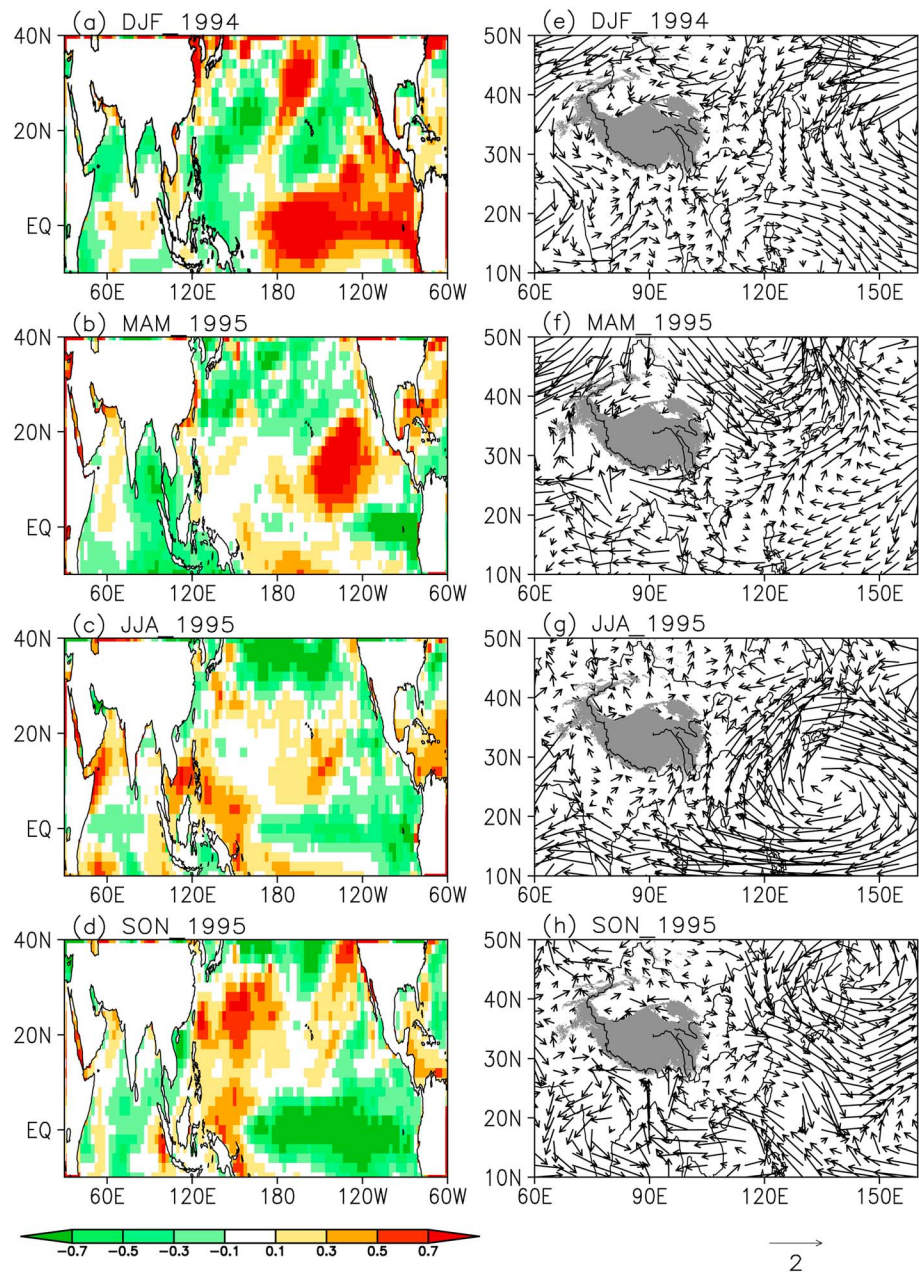
Figure 6. The horizontal distribution of (a–d) skin temperature anomalies ( ^{\circ}\text{C} ) and (e–h) wind anomalies at 850 hPa based on the assimilated meteorological data ( \text{m s}^{-1} ) during El Niño Modoki event 1994/1995.
